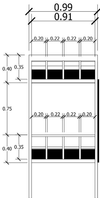
HEADBOARD DETAILS
