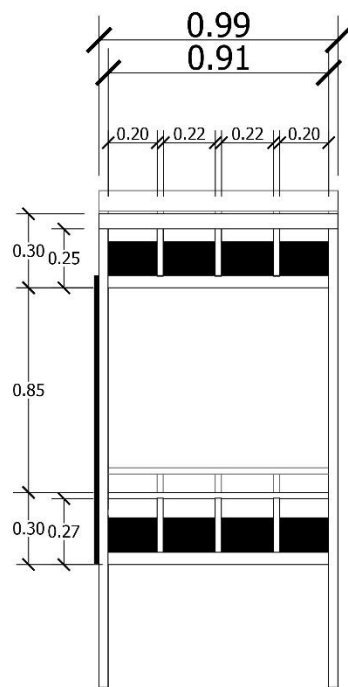
FOOT BOARD DETAILS
