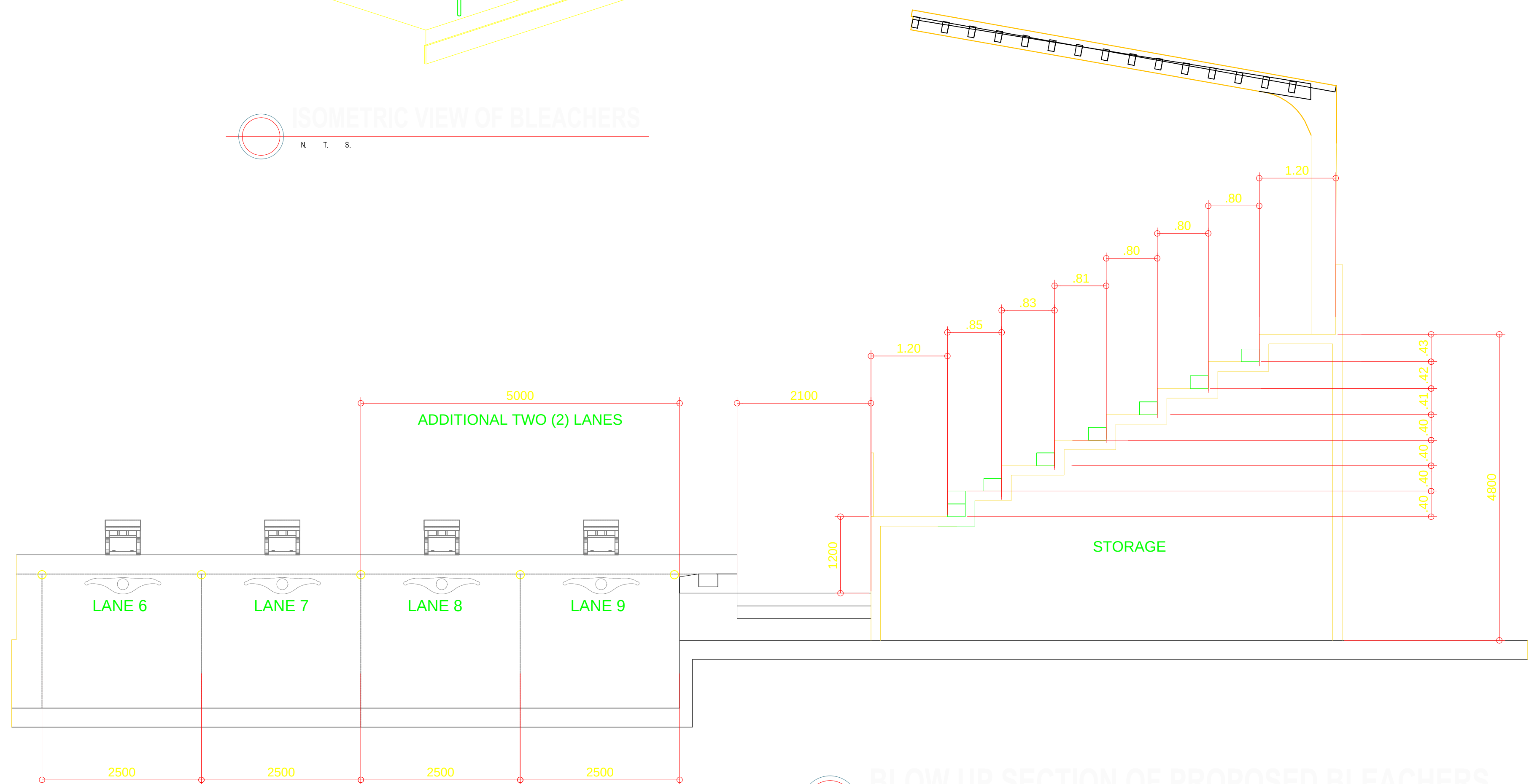
BLOW UP SECTION OF PROPOSED BLEACHERS SCALE 1 : 50 MTS.
