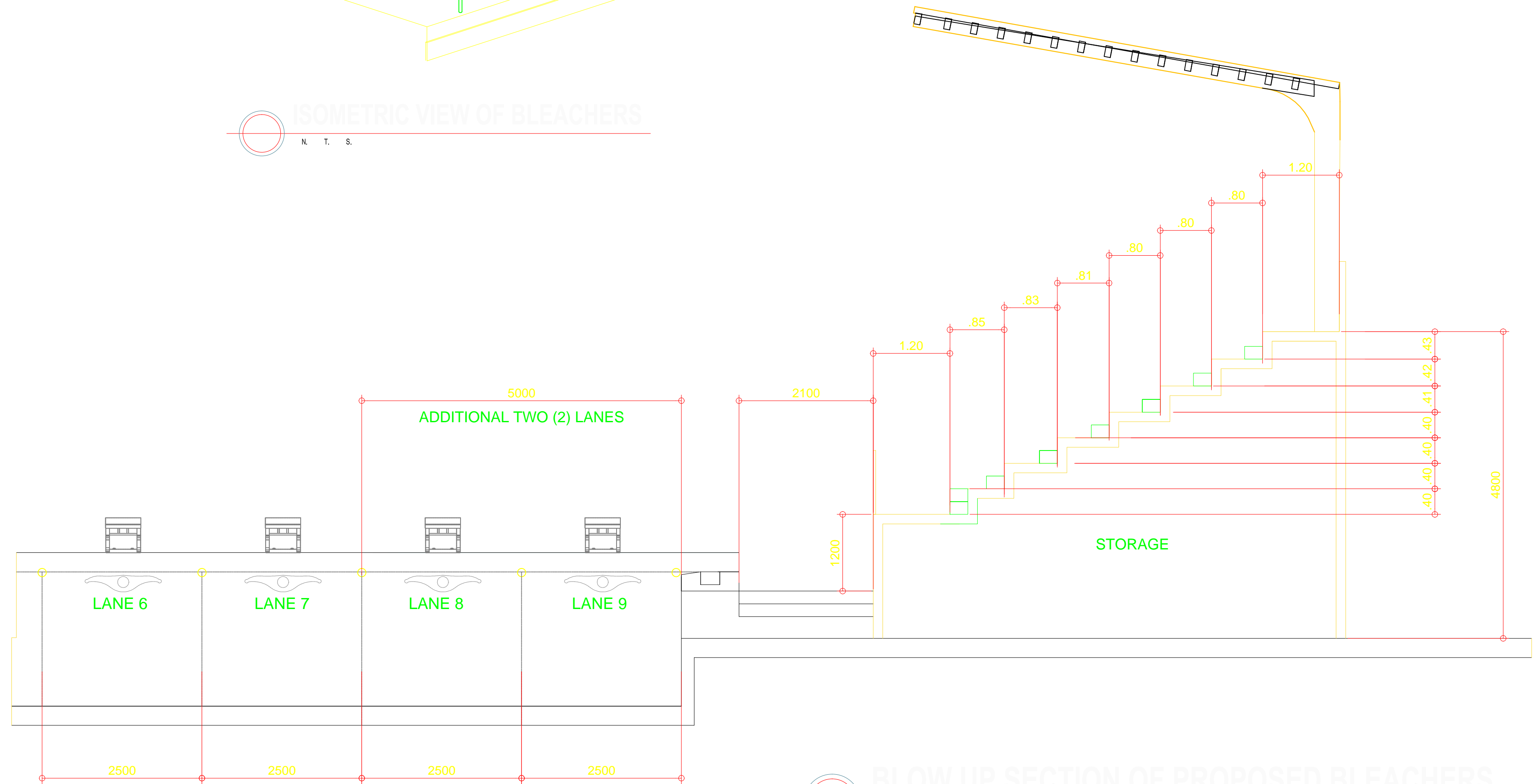
BLOW UP SECTION OF PROPOSED BLEACHERS
