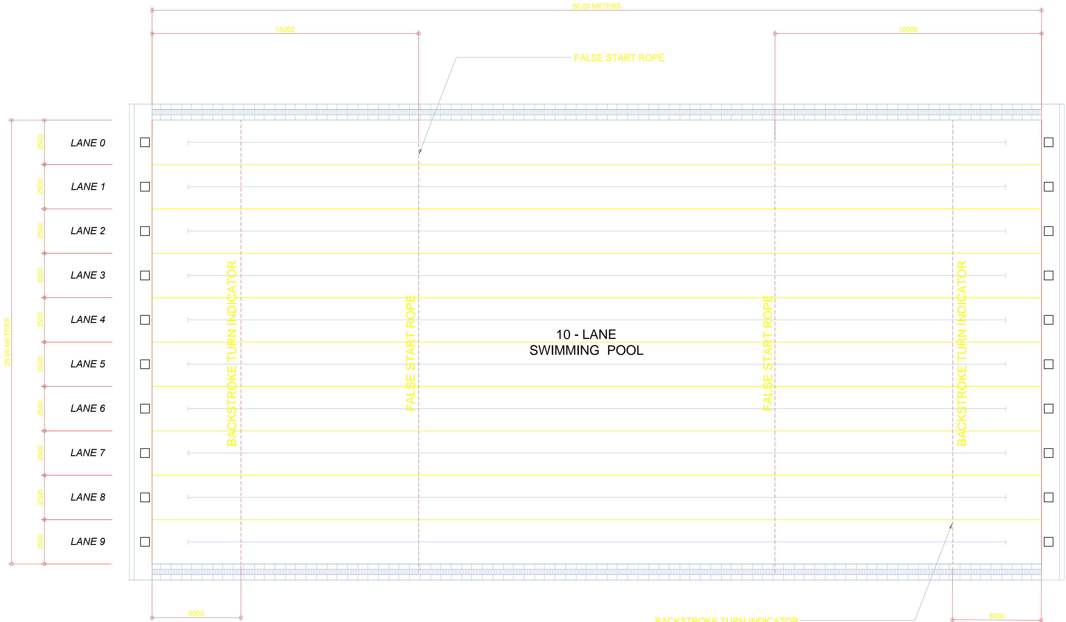
LOCATION OF FALSE START AND BACKSTROKE TURN INDICATOR SCALE 1:100 MTS.
