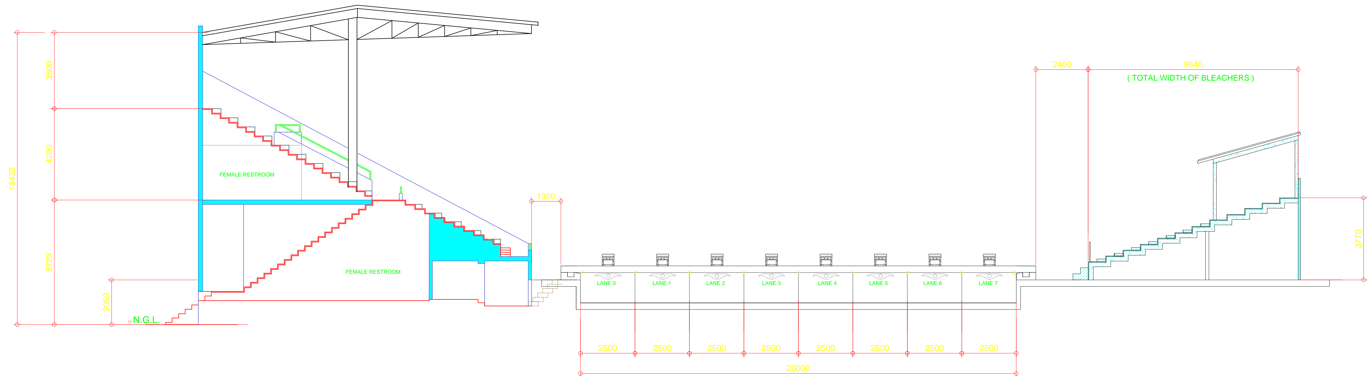
EXISTING CROSS SECTION OF AQUATIC CENTER SCALE 1:20 MTS.
