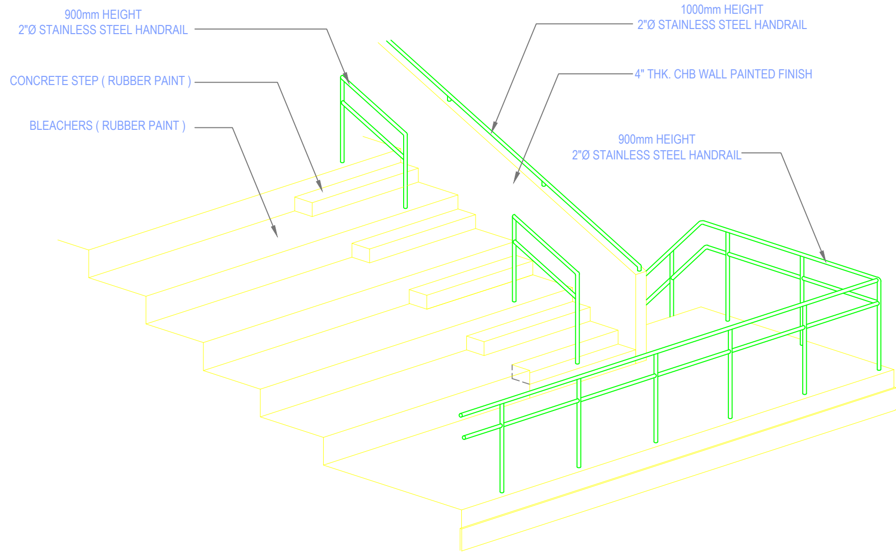
ISOMETRIC VIEW OF BLEACHERS
