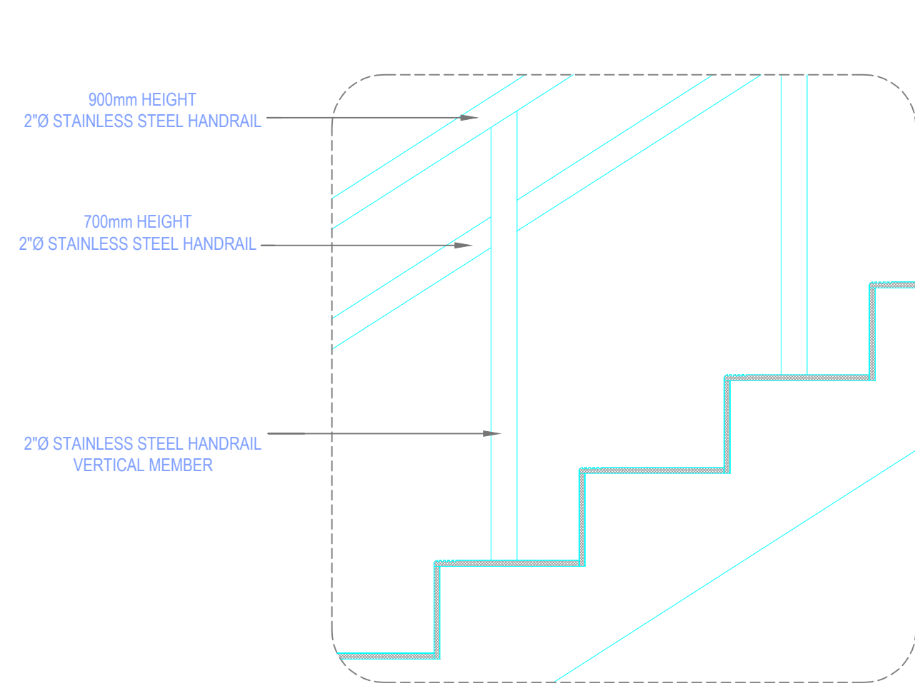
DETAIL OF RAILING
